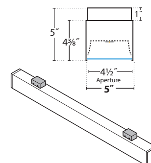
WMU1 — SURFACE
