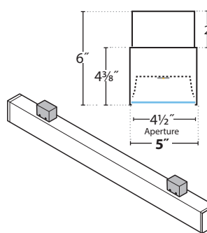
WMU2 — SURFACE
