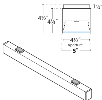
WMU — SURFACE
