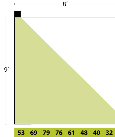
Footcandles along the floor
